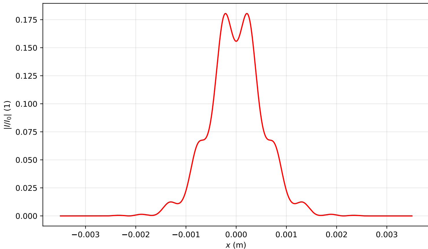
Intensity profile I(x, y = 0, z = 3.662)/I_0 , P_{in}=1.0P_{cr} , artificial time
